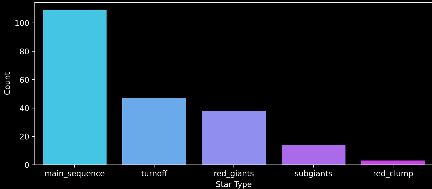
APOGEE DR17 Field: [074+57_MGA] Count plot of Star Type
