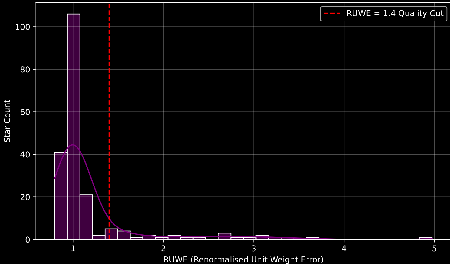
GAPOGEE DR17 Field [074+57_MGA] RUWE Distribution (n= 198)
