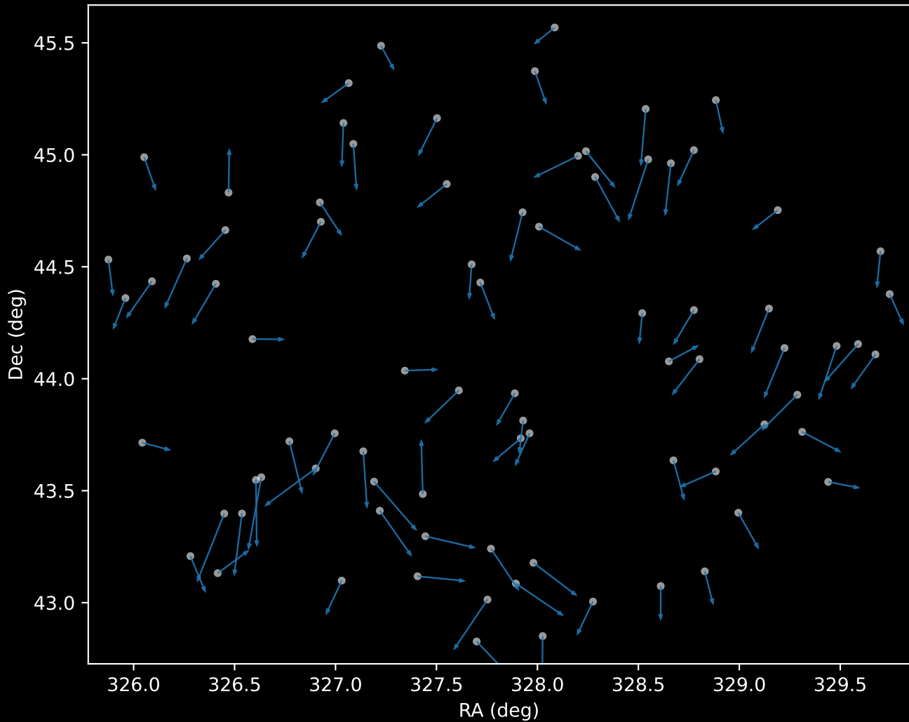
APOGEE DR17 Cluster 0 Proper Motion Vectors (n=82)
