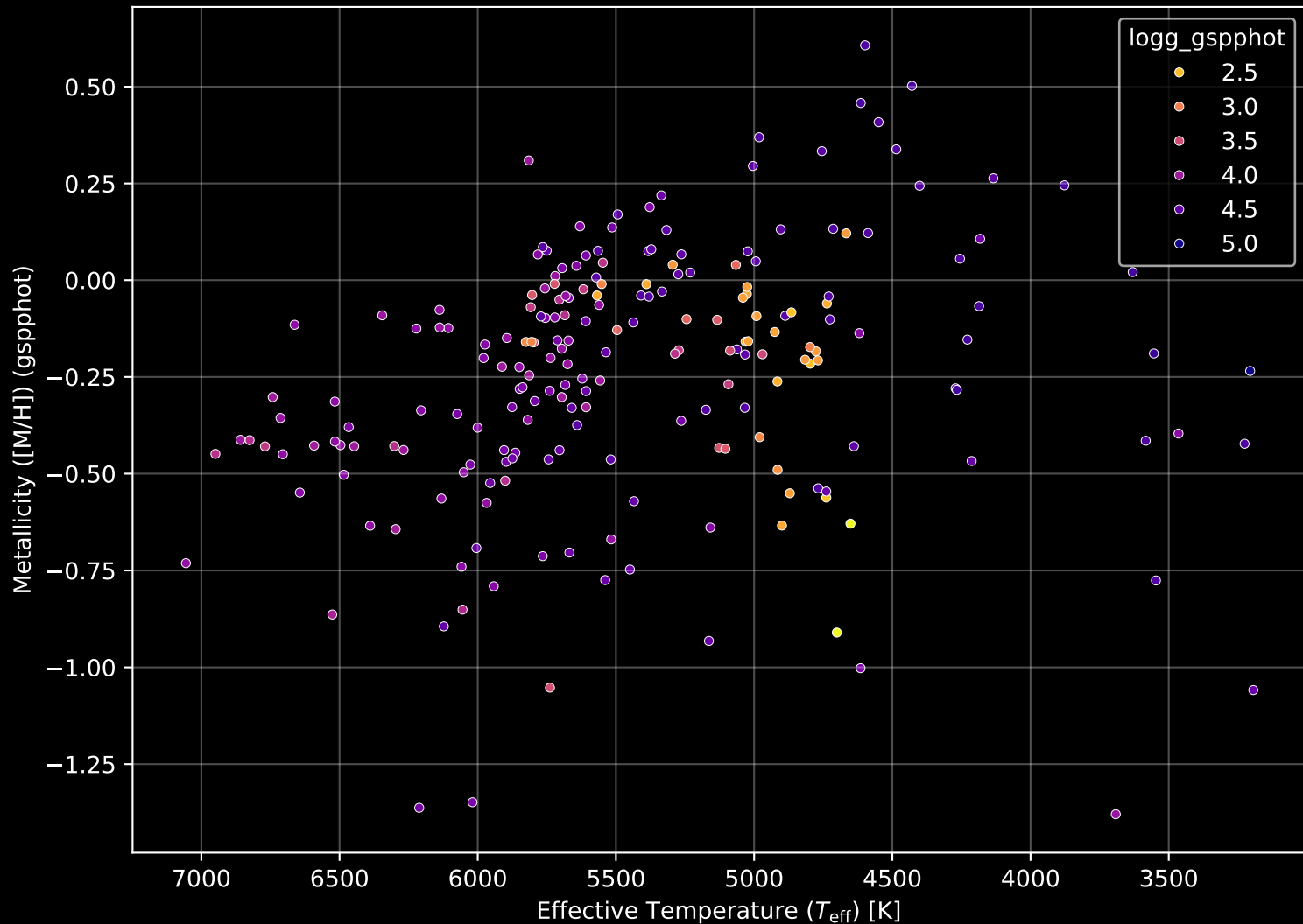
APOGEE DR17 Field: [074+57_MGA] Stellar Population Parameters (n= 211)
