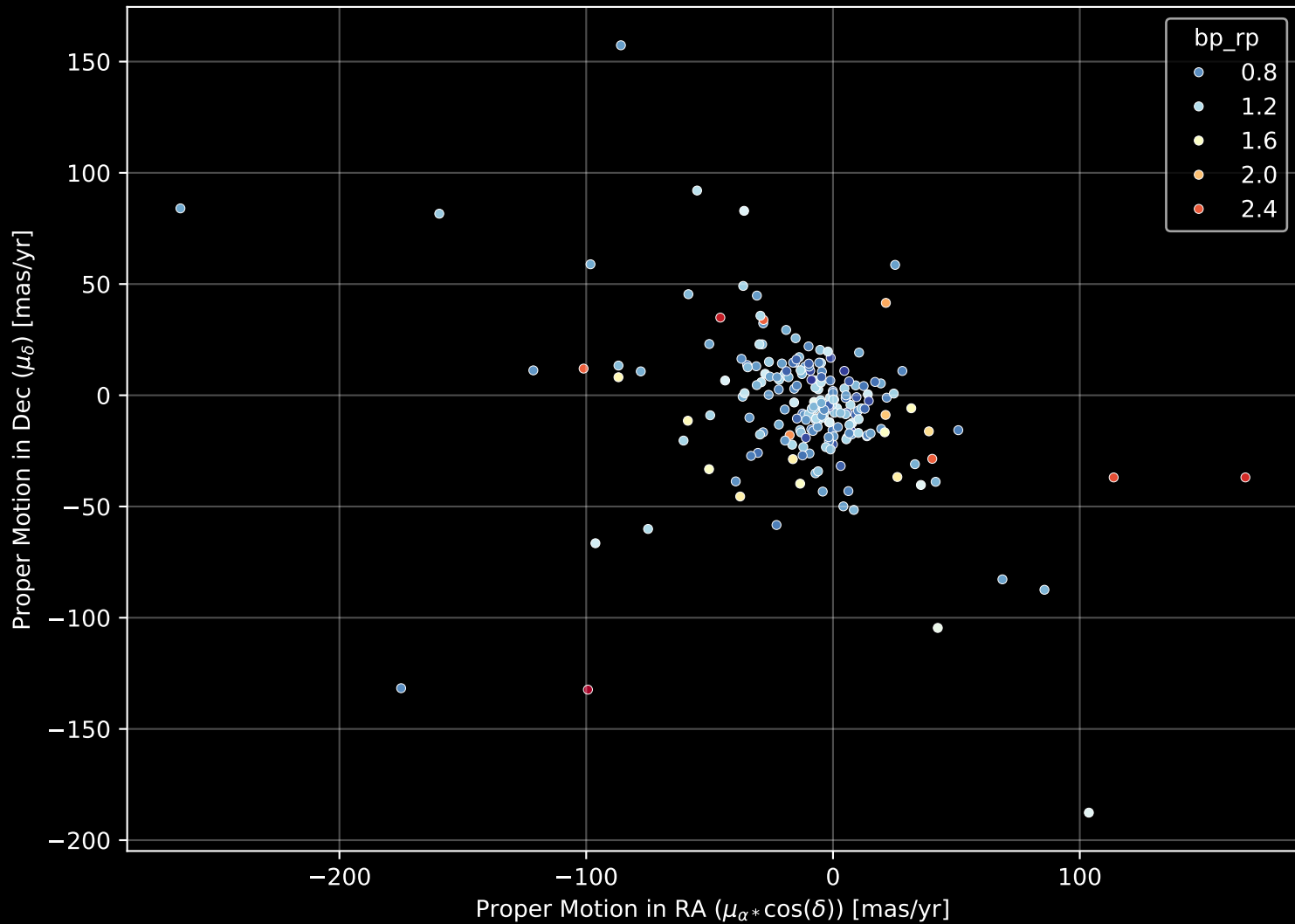
APOGEE DR17 Field: [074+57_MGA] Proper Motion Diagram (n= 211)
