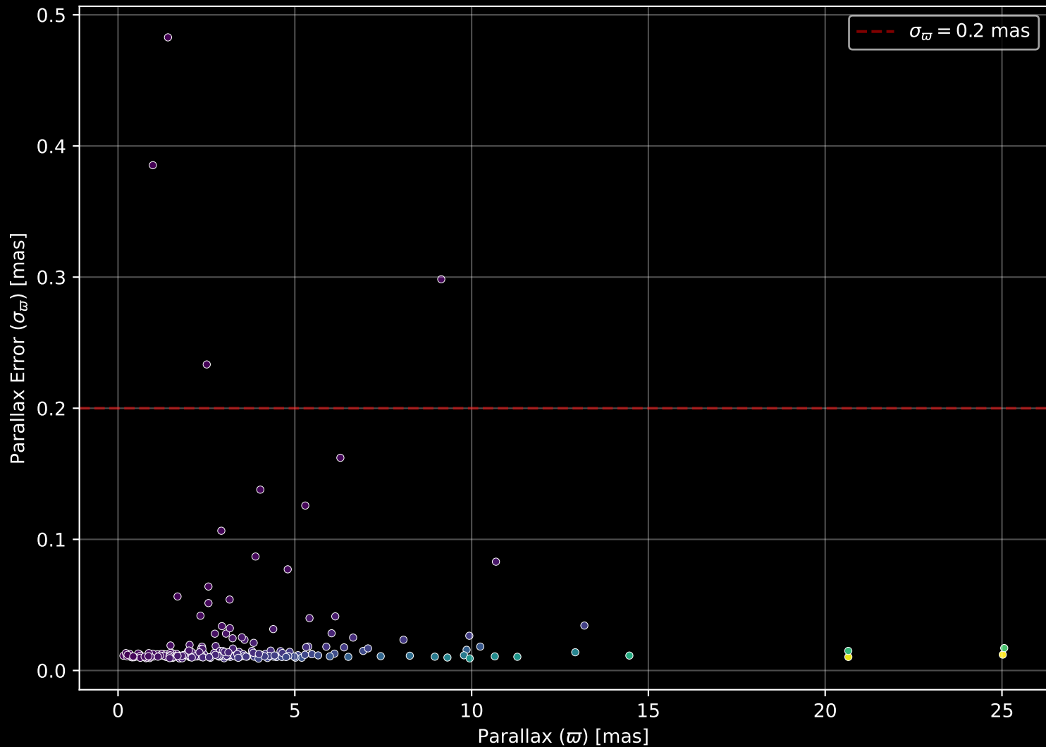
APOGEE DR17 Field: [074+57_MGA] Parallax Quality (n= 211)
