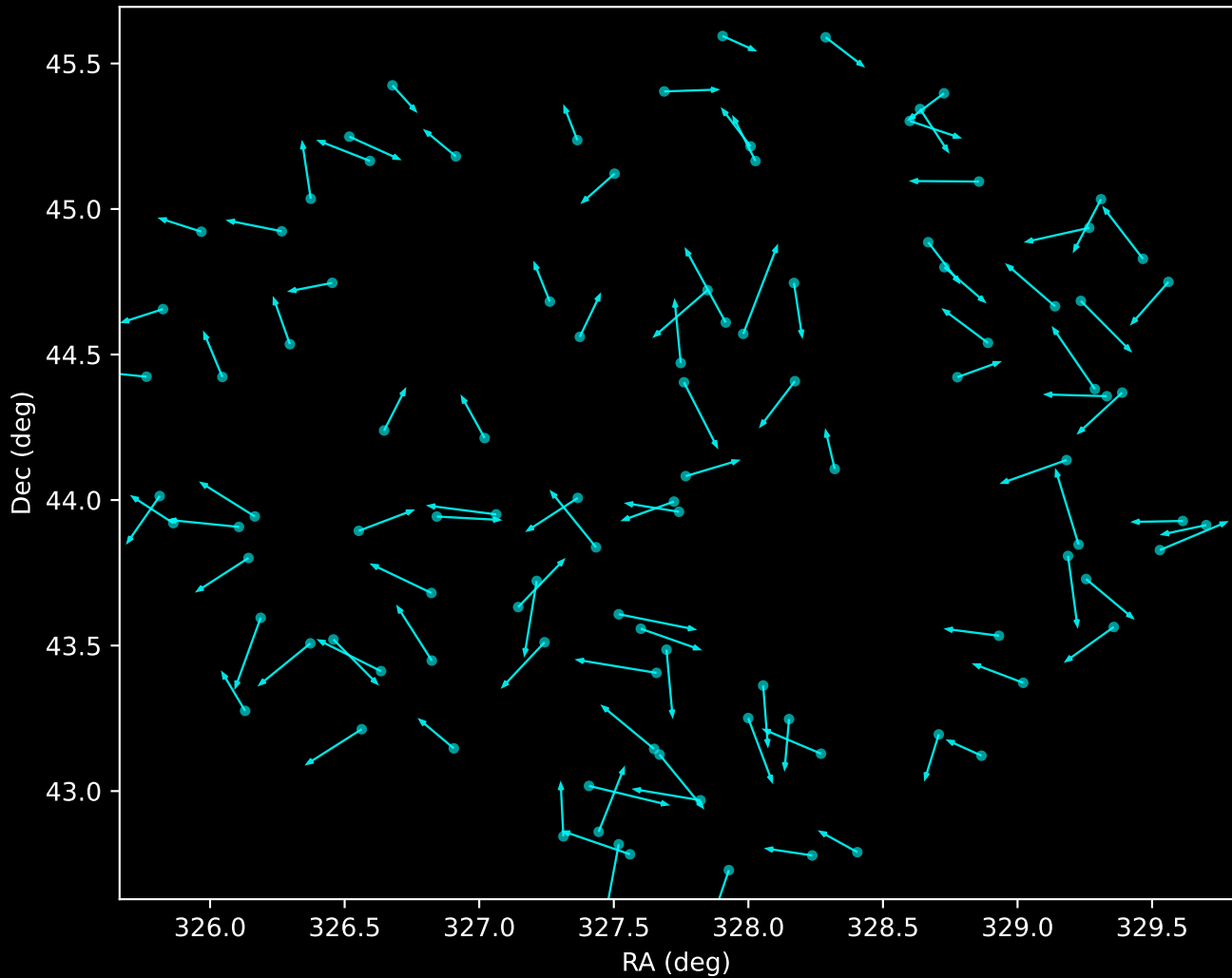
APOGEE DR17 Noise Stream Proper Motion Vectors (n=104)
